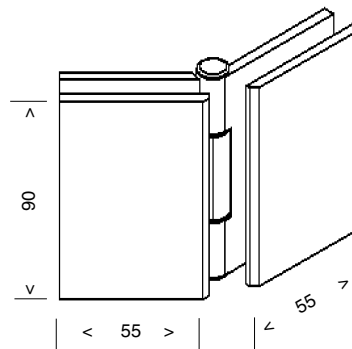
MF2-BF GLASS TO GLASS BIFOLD HINGE
