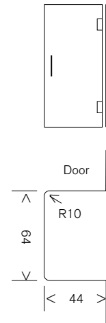
MF1-90 WALL MOUNT HINGE 90° FIXING
