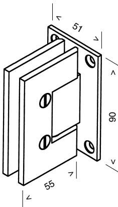
MF1 WALL MOUNT HINGE
