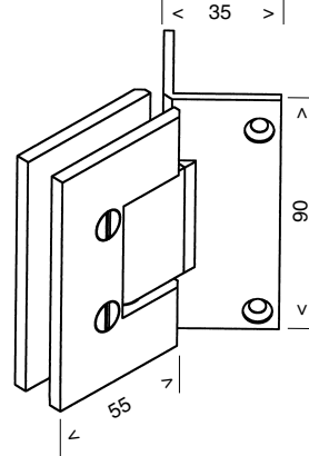
MF1-90 WALL MOUNT HINGE 90° FIXING
