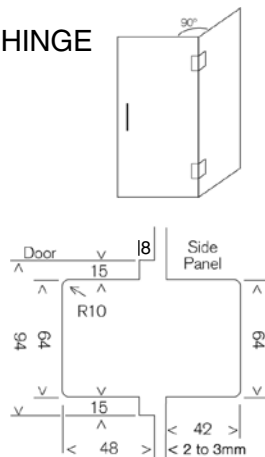
MF2-BF GLASS TO GLASS BIFOLD HINGE
