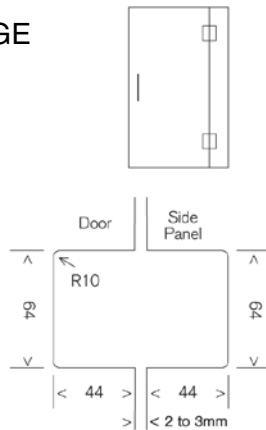
MF2-90 GLASS TO GLASS 90° HINGE
